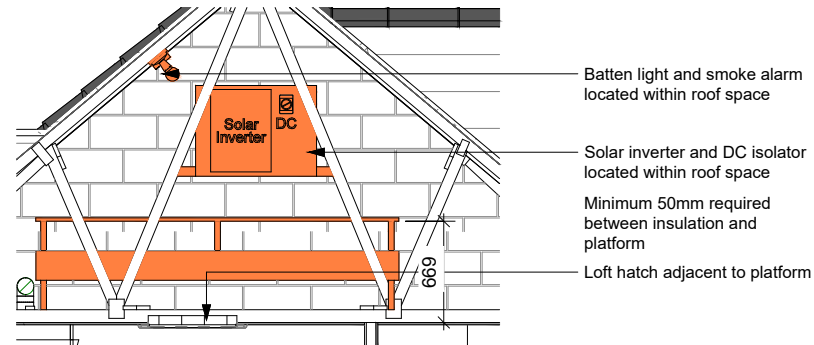
2 Solar Invertor (2021 Only) 1 : 50
