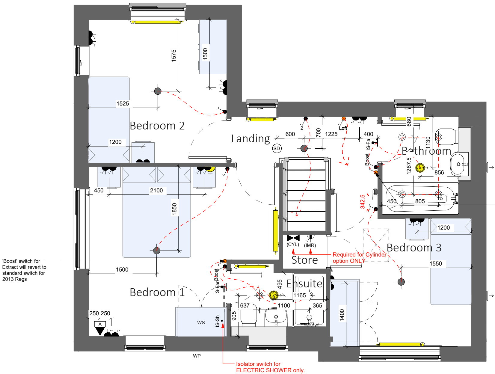
1 First Floor Electrical GA 1 : 50
